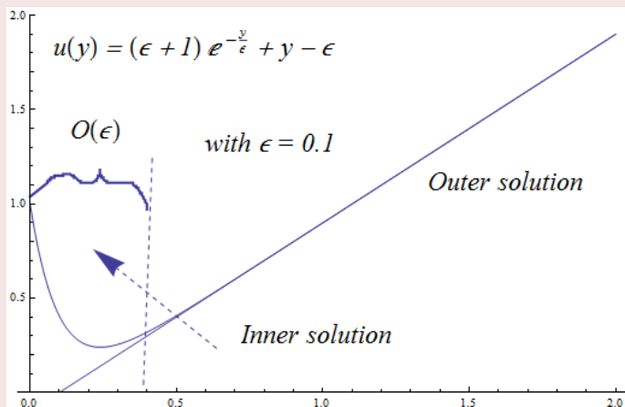
Figure 11.2: Plot of exact solution to simple first order ill conditioned LDE.
