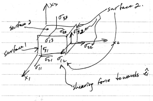
Figure 3.8: Strain components on a 3D volume.
