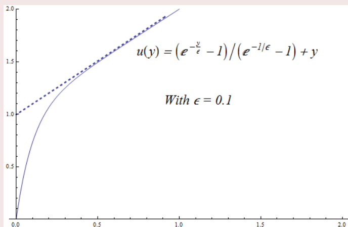
Figure 11.3: Plot of our ill conditioned second order LDE.
