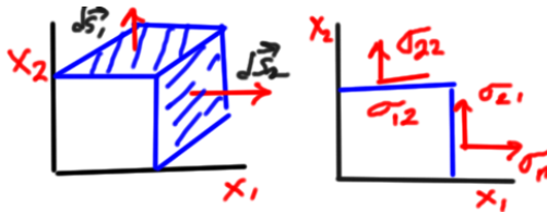
Figure 3.5: 2D stress tensor.
